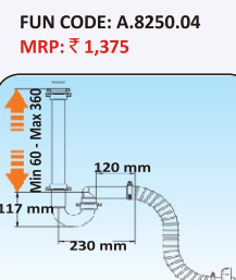
MODEL TYPE: LIRA 'P' TRAP FINISH: WHITE & SINGLE BOWL
