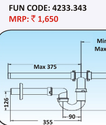
MODEL TYPE: LIRA BWD 'P' TRAP FINISH: WHITE & DOUBLE BOWL
