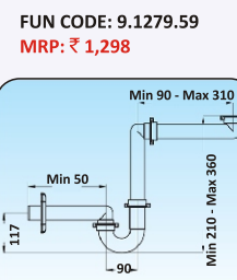
MODEL TYPE: LIRA SPAZIO 'P' TRAP FINISH: WHITE & SINGLE BOWL
