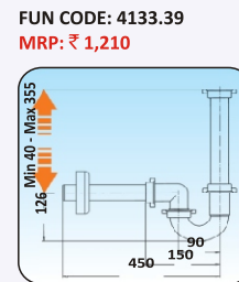
MODEL TYPE: LIRA 'P' TRAP FINISH & TYPE: WHITE & SINGLE BOWL
