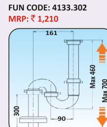
MODEL TYPE: LIRA 'S' TRAP FINISH & TYPE: WHITE & SINGLE BOWL
