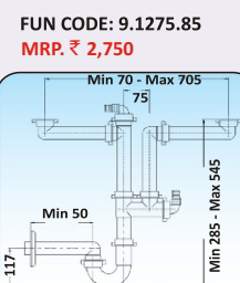
MODEL TYPE: LIRA SPAZIO 'P' TRAP FINISH: WHITE & DOUBLE BOWL
