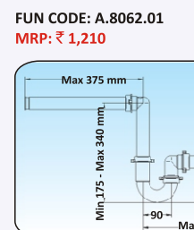
MODEL TYPE: LIRA BWD 'P' TRAP FINISH & TYPE: WHITE & SINGLE BOWL
